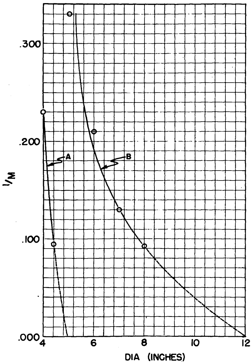
FIG 7 1/M AS A FUNCTION OF DIAMETER OF U-235 PSEUDOSPHERE OF A 100% DENSITY & B 50% DENSITY IN WATER TANK
